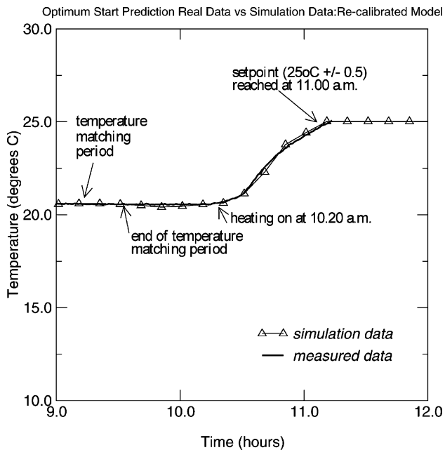
Fig. 8. Model prediction vs. monitored data after re-calibration.
