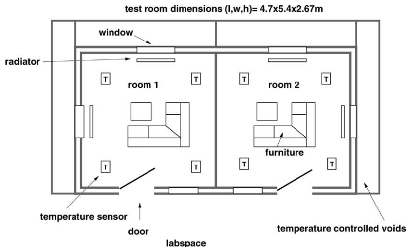
Fig. 5. Plan view of the test rooms and voids.
