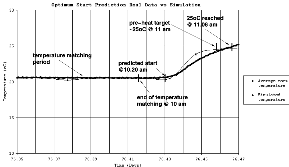
Fig. 7. Optimum start experiment—model prediction vs. monitored data.
