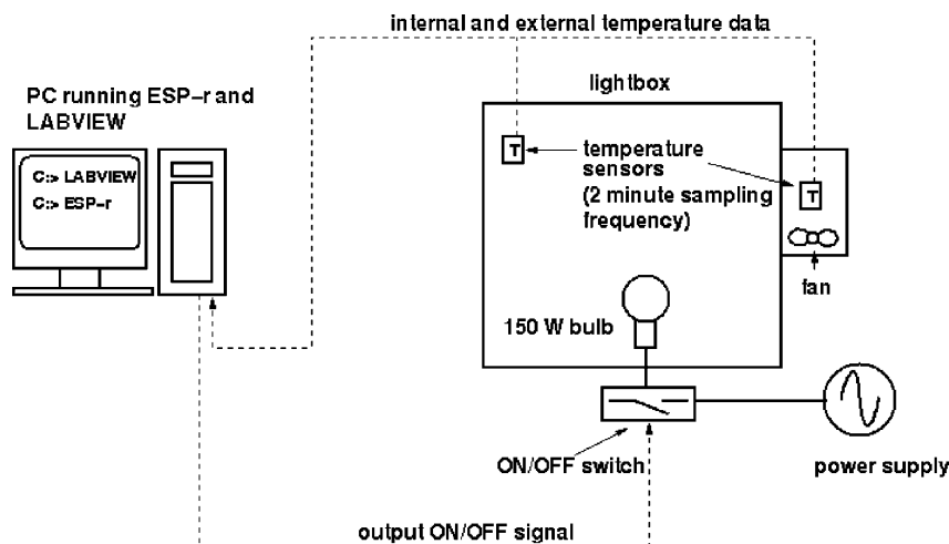
Fig. 3. Preliminary experimental configuration.
