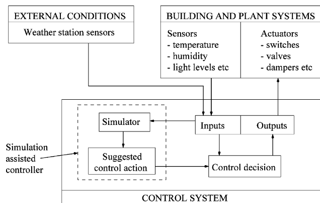
Fig. 1. Simulation-assisted control in BEMS.
