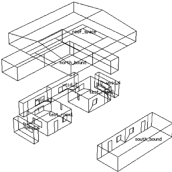
Fig. 6. Exploded view of the ESP-r model.
