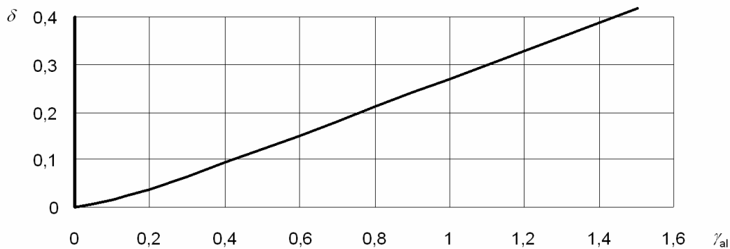
Figure E.3 — Ratio \delta of the accumulated internal-external temperature difference when the ventilation is on, to its value over the whole calculation step, as a function of the gain/load ratio of the air layer, \gamma_{al}
