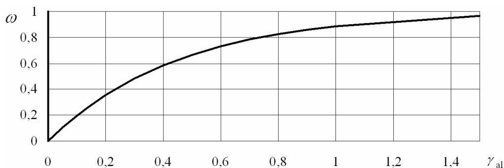
Figure E.4 — Ratio \omega of the total solar radiation falling on the element when the air layer is open to the total solar radiation during the calculation step, as a function of the heat balance ratio of the air layer, \gamma_{al}
