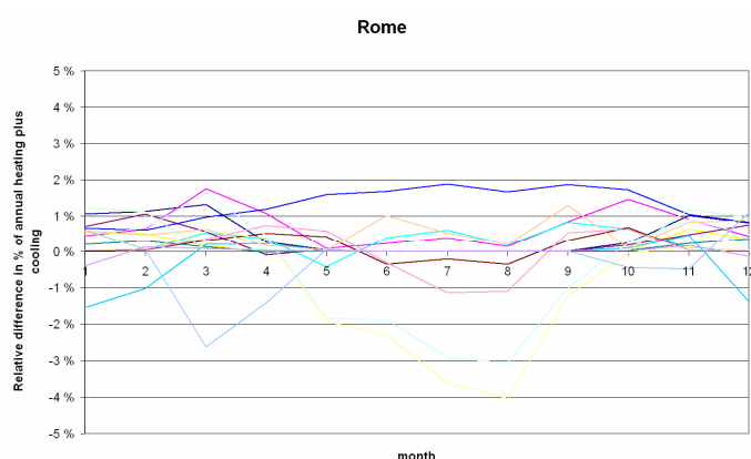
Figure H.3 — Summary of results for Rome
