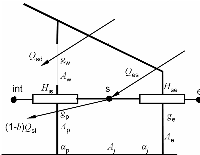
Figure E 1 — Attached sunspace with solar heat gains and heat transfer coefficients, and electrical equivalent network; detailed method
