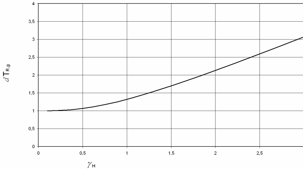
Figure I.1 Example of curve for the relative overtemperature dT_{R,g} as function of gain-loss ratio \gamma_H (for a = 2,12 ).
