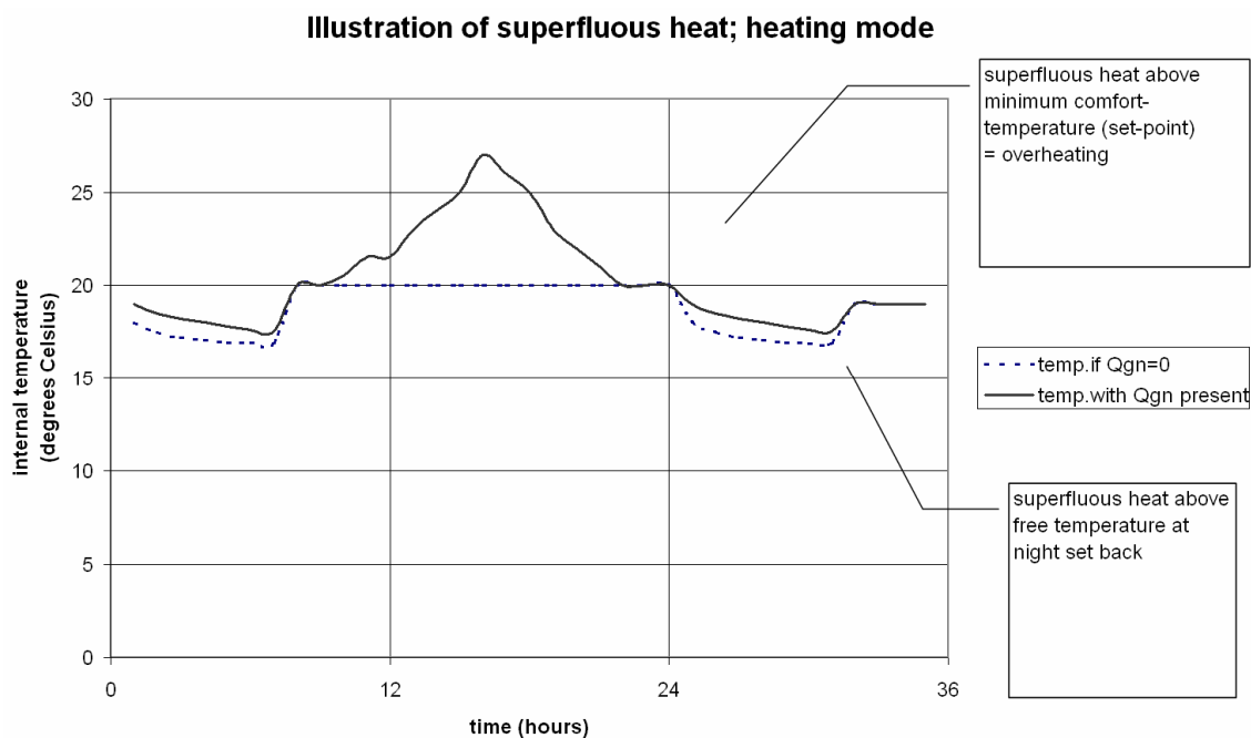
Figure I.2 — Illustration of daily pattern of indoor temperature with and without heat gains
