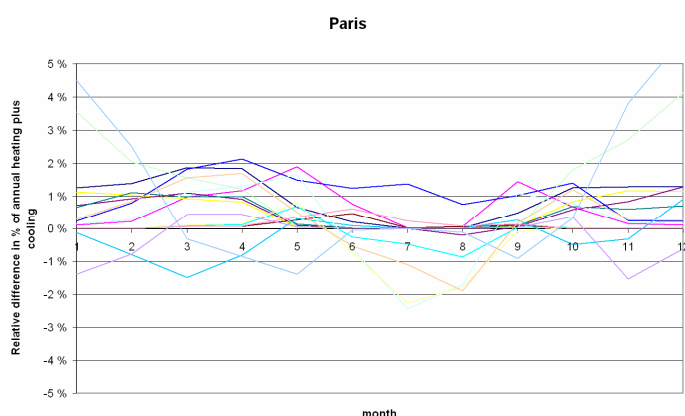
Figure H.2 — Summary of results for Paris
