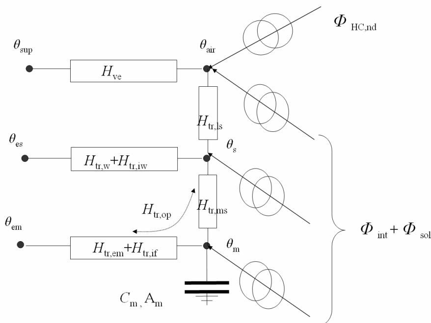
Figure B.1 — Modified RC network
