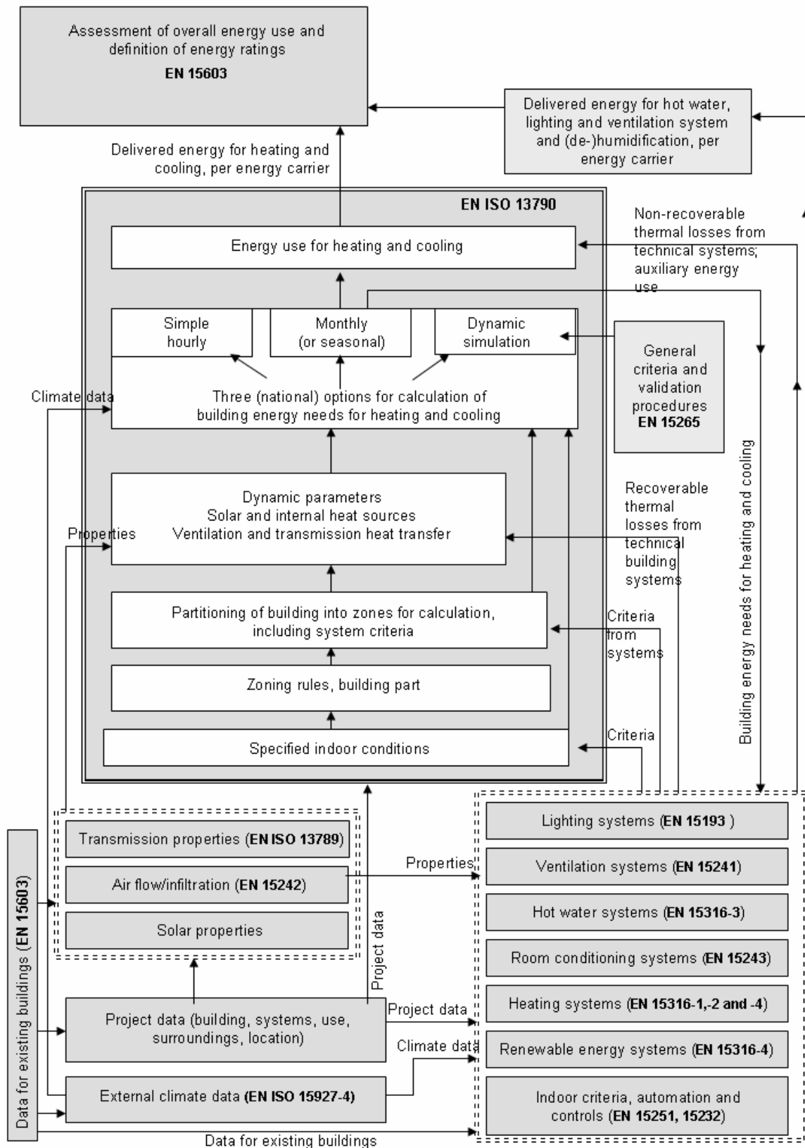
Figure A.1 — Flow chart of calculation procedure and links with other standards for the CEN area
