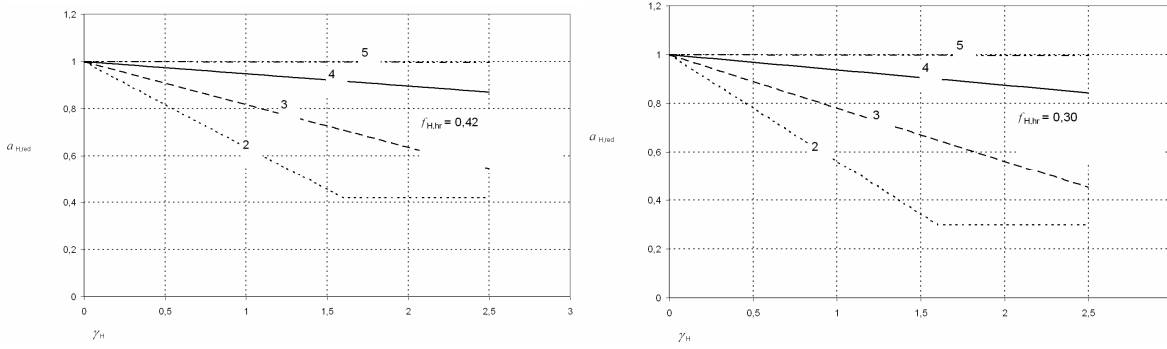
Fig.8.a: f_{H,hr} = 0,42 : normal heating during 5 days, 14 hrs per day
