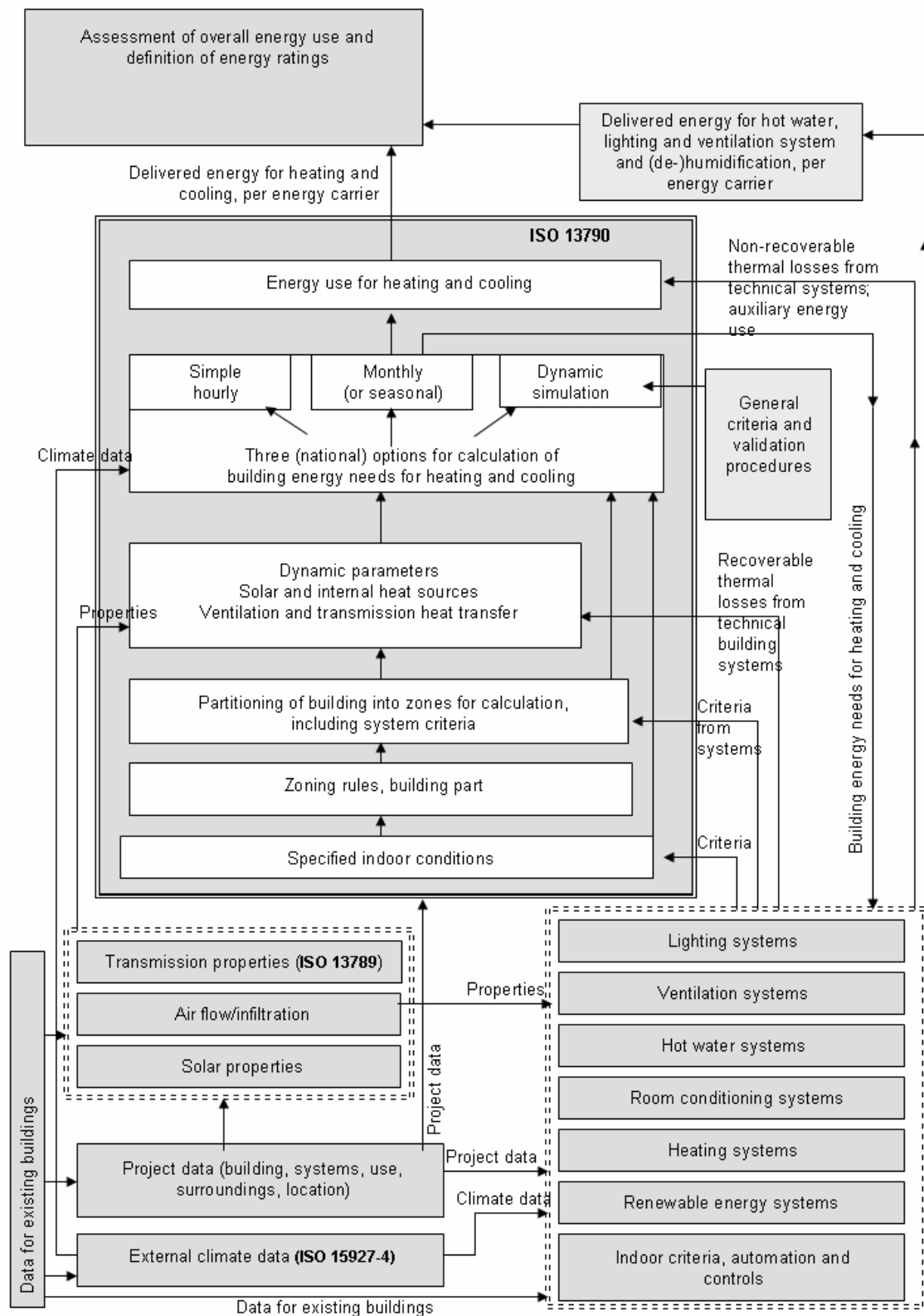
Figure 1 — Flow chart of calculation procedure and links with other standards
