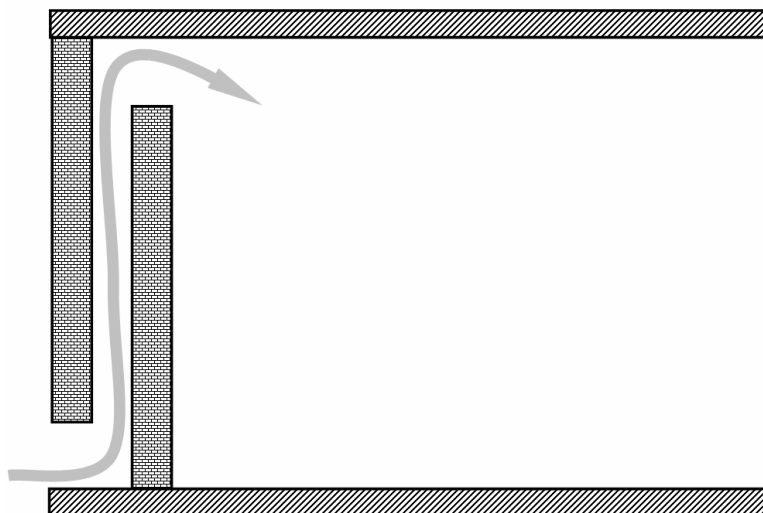
Figure E.5 — Air path in the wall
